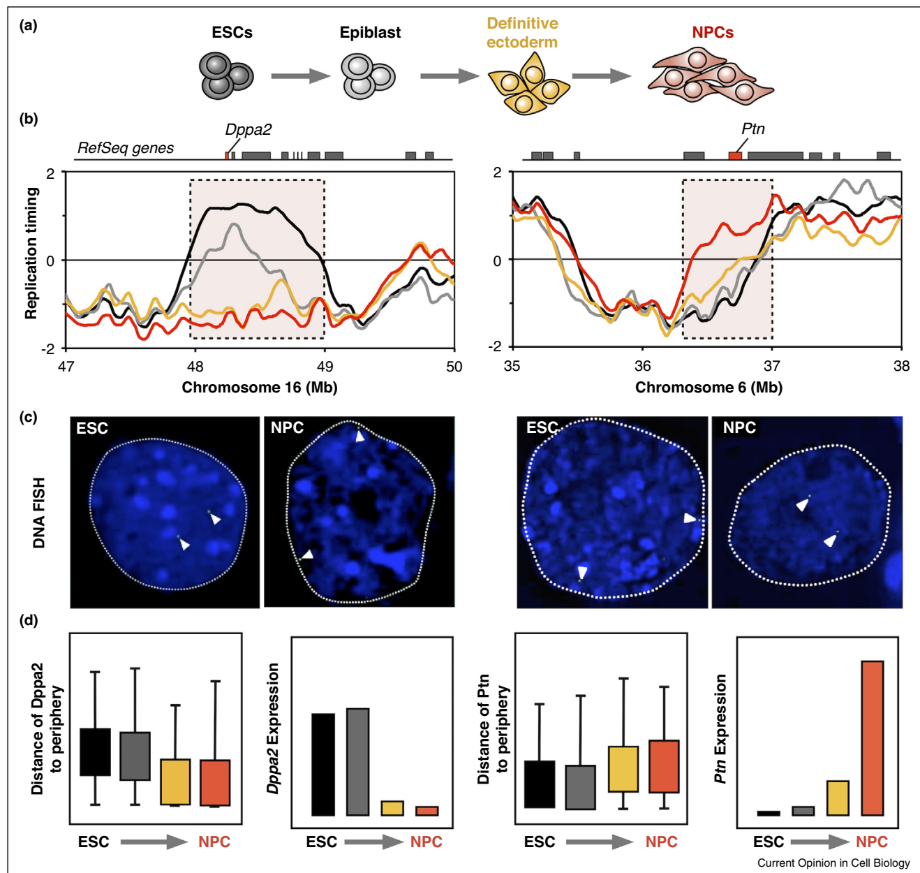
RT changes are associated with nuclear re-localization and gene expression. (a) Schematic depiction of neural differentiation (NPCs) from mouse embryonic stem cells (ESCs). (b) RT changes during neural differentiation. Location of Dppa2 and Ptn genes are shown at the top. (c) Nuclear re-localization of Dppa2 and Ptn domains during neural differentiation visualized by DNA FISH. (d) Measurements of radial nuclear positioning (distance to the nuclear periphery) and gene expression of Dppa2 and Ptn genes. Colors in the graphs represent the distinct differentiation stages as shown in (a). Data and FISH images were obtained from [12].
